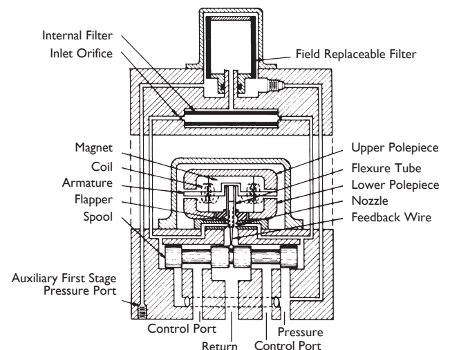
Figure 1 Moog Series (G)730K
